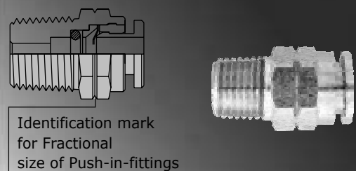
SEALEXCEL Fractional size stainless steel Push-In-Fittings
